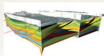
▲ Geological model, Rockwork output
